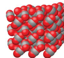
carbon dioxide
