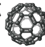
Buckyball
