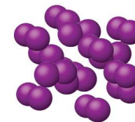
iodine
