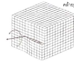
Screw dislocation
