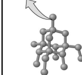
diamond
