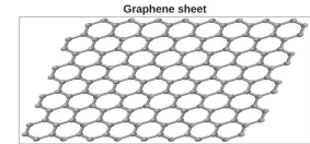
Graphene sheet
