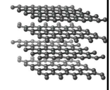
Stacked sheets
