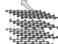
graphite
